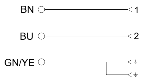
ELECTRICAL DIAGRAM 00
